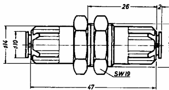
Bulkhead Coupling 56030
